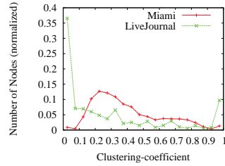
Fig. 2. Clustering coefficient distributions.
